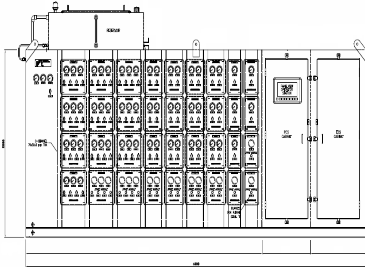
FRONT VIEW
